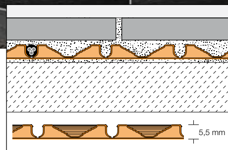
Schlüter®-DITRA-HEAT
